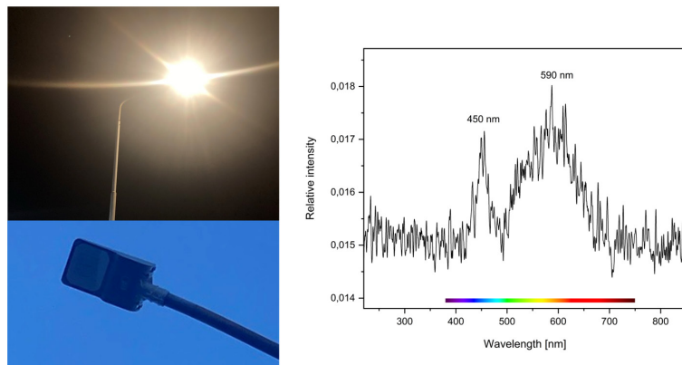
Figure 4: Luminaire 6 in nighttime and daytime and its emission spectrum, which is noisier than others, with smaller peak at 450 nm and broader at approximately 590 nm
